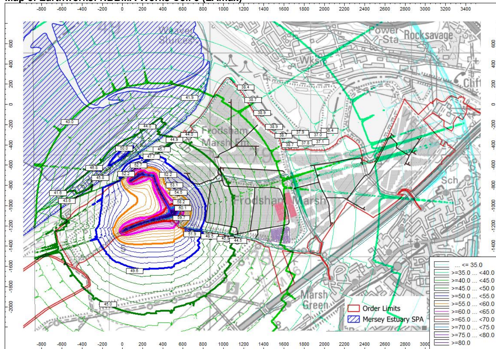
Map 5: Earthworks: NBBMA Works Cell 3 (LAmox)
